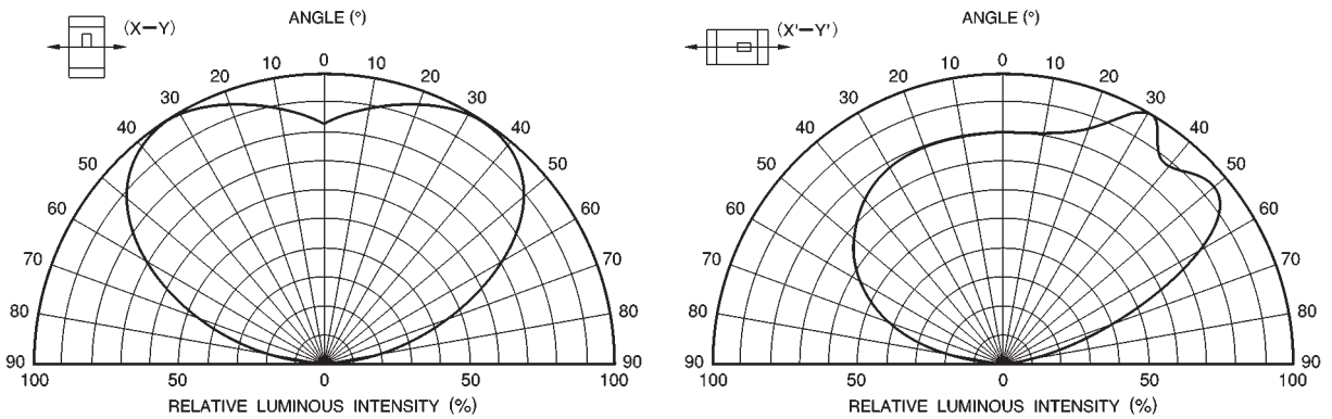
Fig. 1 Directional pattern
