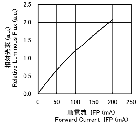
■ 順電流-相対光束特性 Forward Current vs. Relative Luminous Flux
